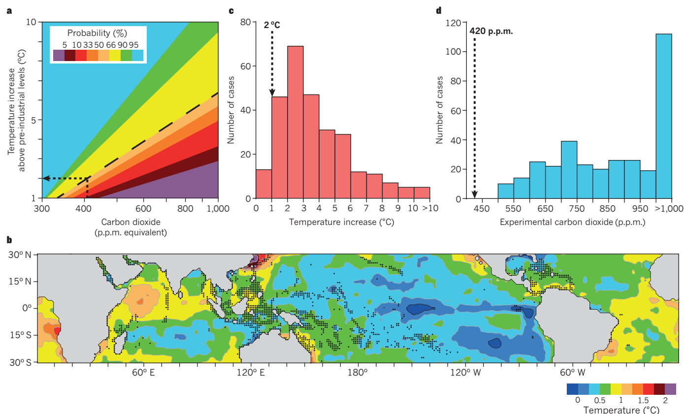
Figure 1 | The climate gauntlet faced by coral reefs. a , The relationship between stabilized concentrations of atmospheric carbon dioxide and stabilized increases in global average temperature above pre-industrial levels. The dashed line indicates a probability of 66%. Adapted from ref. 95. b , Global trends in tropical sea surface temperature from 1880 to 2015. Rates of warming of annual average sea surface temperature were calculated on the basis of linear trend analysis of the HadISST data set 96,97 for all 1° latitude by 1° longitude boxes between 30.5° N and 30.5° S
