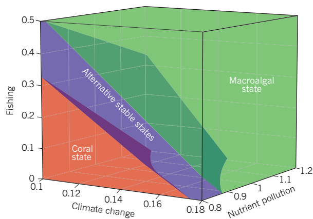
Figure 3 | The modelled response of coral reefs to multiple anthropogenic drivers. Depending on the strength and interaction between certain anthropogenic drivers (climate change, nutrient pollution and fishing), three outcomes are possible: when the drivers are weak, healthy coral-dominated assemblages form (coral state, red); when the drivers are strong, a state dominated by macroalgae with few corals forms (green); and when the drivers are intermediate, alternative states occur (purple). Interfaces between the coral, alternative and macroalgal states represent the tipping points or thresholds for each combination of drivers. The coral state collapses if the stress from any single driver is too strong and is eliminated entirely by the cumulative impacts of multiple drivers. The width and shape of the region of alternative stable states depends on the strength of interacting feedbacks. (See Supplementary Note 1 for further details about the model.)
