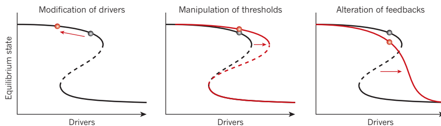
Figure 4 | A heuristic model of future management options for coral reefs. The x-axis represents one or more drivers of change, including climate change, pollution and overfishing, and the y-axis is the resultant state (at equilibrium) of the social or ecological system. Dashed lines indicate the intermediary range of drivers in which both healthy and degraded states are possible. Current stable states of the system are shown as black curves, whereas the red curves represent various potential approaches to reef management. The black and red dots indicate the state of the
